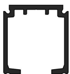
Single Upper Running Track Type 1280 Product # 891280A210
