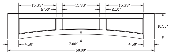
60" Flat Panel Valance
