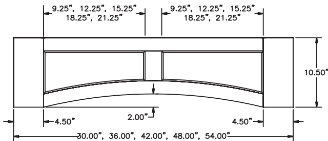
30", 36", 42", 48" and 54" Flat Panel Valance
