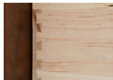
Maple dovetail construction
